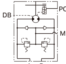
回路図 (CHB型) hydraulic symbol (CHB type)
