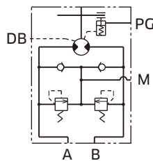
回路図 (CHB型) hydraulic symbol (CHB type)
