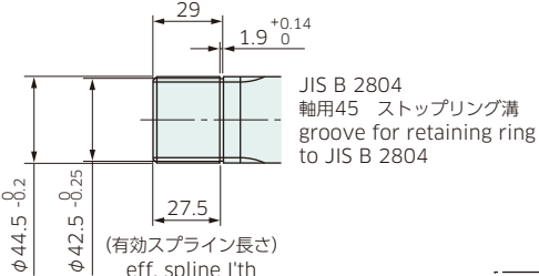
軸端詳細 detail of shaft end
